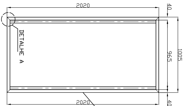
VISTA FRONTAL
